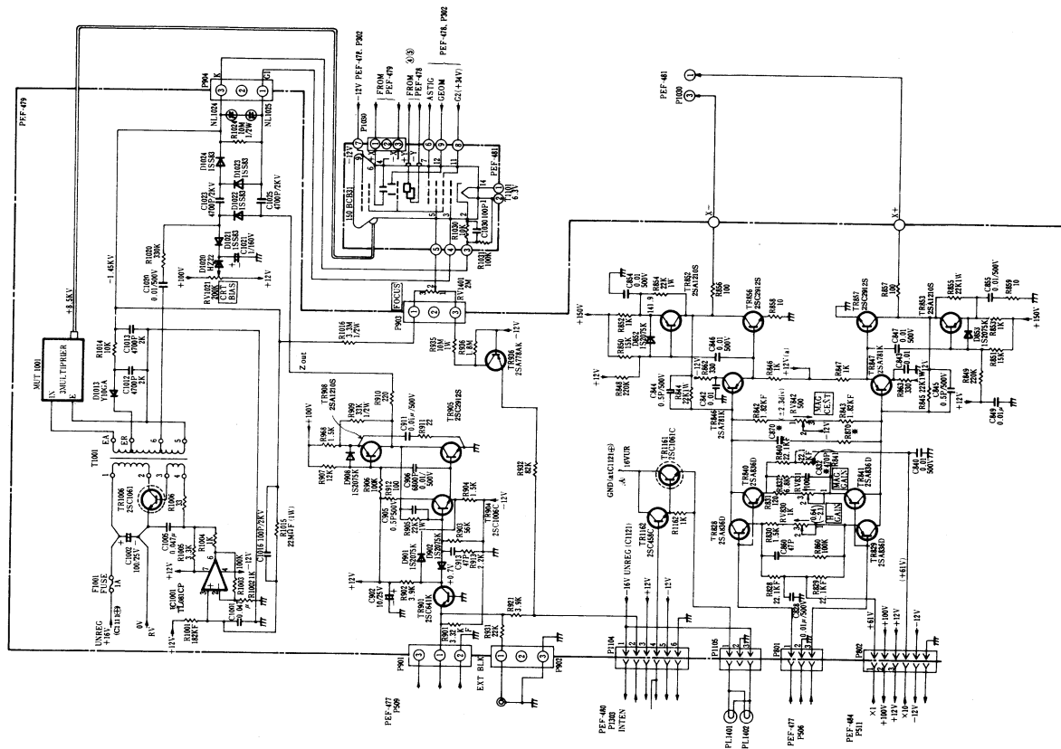
◇ V-650F HIGH VOLTAGE UNIT & Z-AXIS HORIZONTAL AMP
