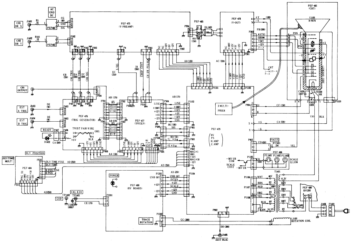
⑨ V-650F WIRE CONNECTION
