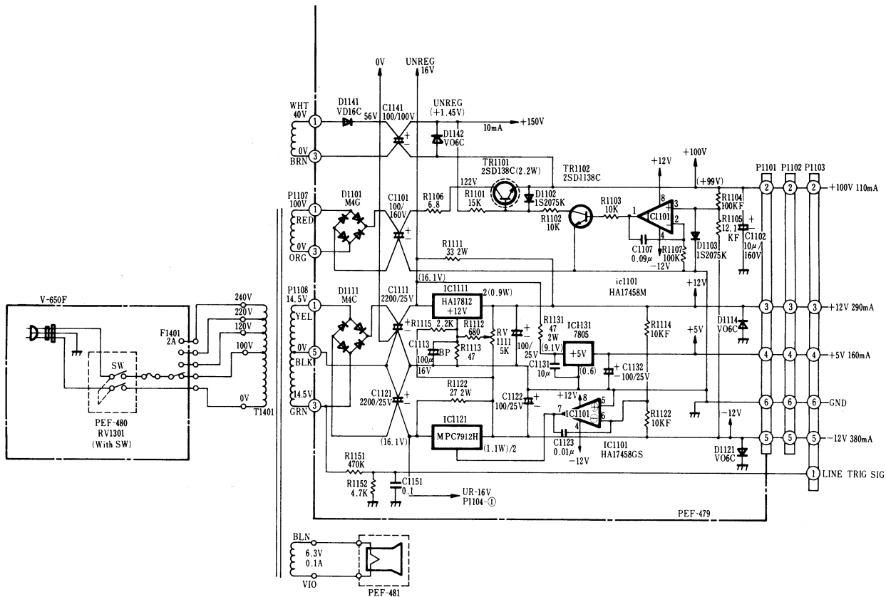
⑥ V-650F POWER SUPPLY
